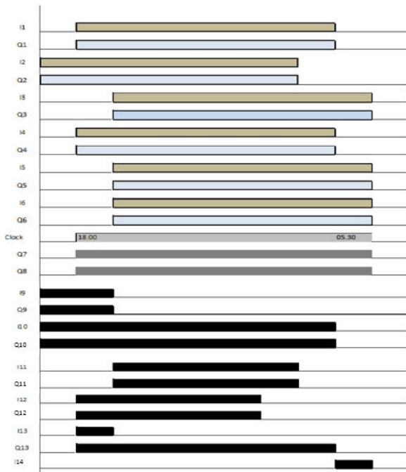
Gambar 8. Hasil Pengujian ( Timing Diagram )
