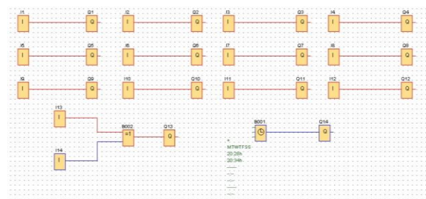
Gambar 7. Function Block Diagram (FBD)
